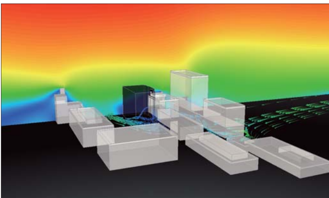
Figure 2: Results of an external wind flow study post-processed in scSTREAM - perspective view (left) and top view (right)
